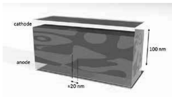
Figure 23: Structure of a Bulk Heterojunction Cell.
