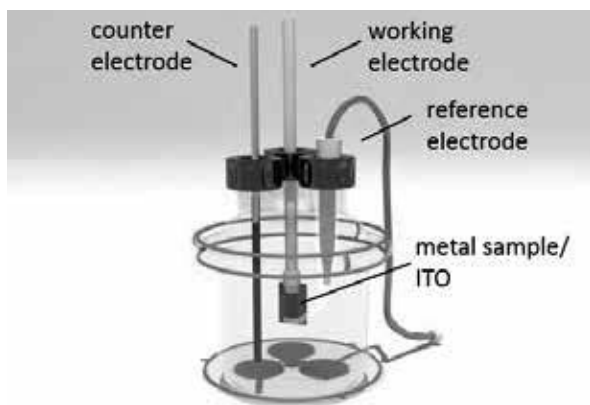
Figure 6: Three-electrode electrochemical cell.
