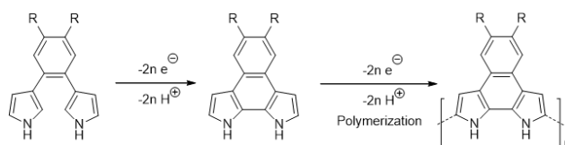
Figure 7: Electrochemical polymerization of a bipyrrrole (11) .
