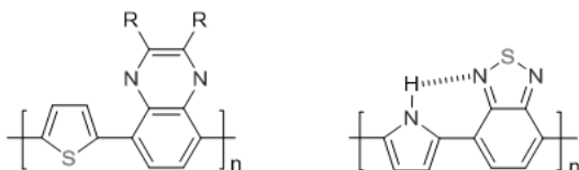
Figure 29: Acceptor-donor copolymers (45) .
