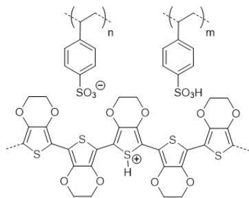
Figure 18: PEDOT:PSS.
