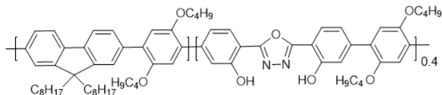
Figure 35: Polymer described by Wang et al. with \text{F}^- selectivity (70) .
