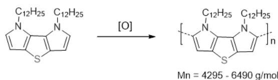
Figure 4: Preparation of a conjugated polymer by chemical oxidation (7) .
