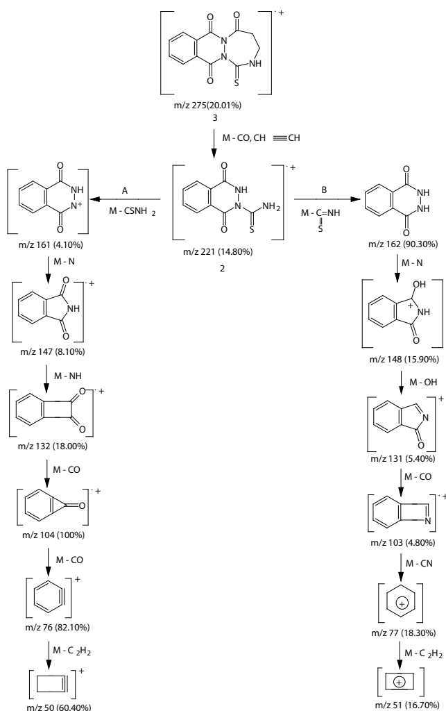
Scheme 2. Main fragmentation pathway of compounds 2 and 3
