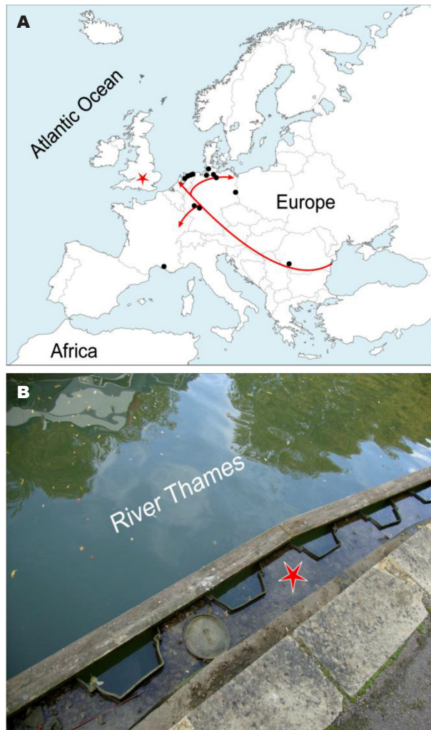
Fig. 1. A. Geographic range of Oligochoerus limnophilus . Black dots, previously known localities for the species (data extracted from literature and the Turbellarian Taxonomic Database [Tyler et al., 2006–2012]). Red star, this study. Red arrows indicate the South Central migration corridor of Pontic–Caspian aquatic invertebrates that connects the Danube and the Rhine water basins through the Main–Danube Canal (Ketelaars, 2004). B. Picture of the habitat at Oxford. Red star: artificial substrate where individuals of O. limnophilus were collected.
