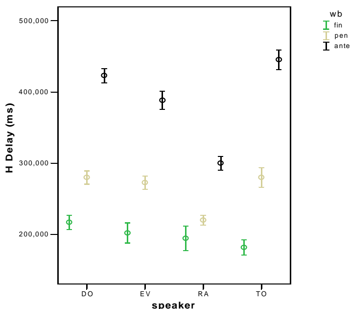
Figure 4. Mean H peak delay (or distance in ms between the H peak relative to the beginning of the accented syllable) as a function of within-word position for all speakers: fin (words with a final accent), pen (words with a penultimate accent) and ante (words with an antepenultimate accent). The bars represent standard errors.
