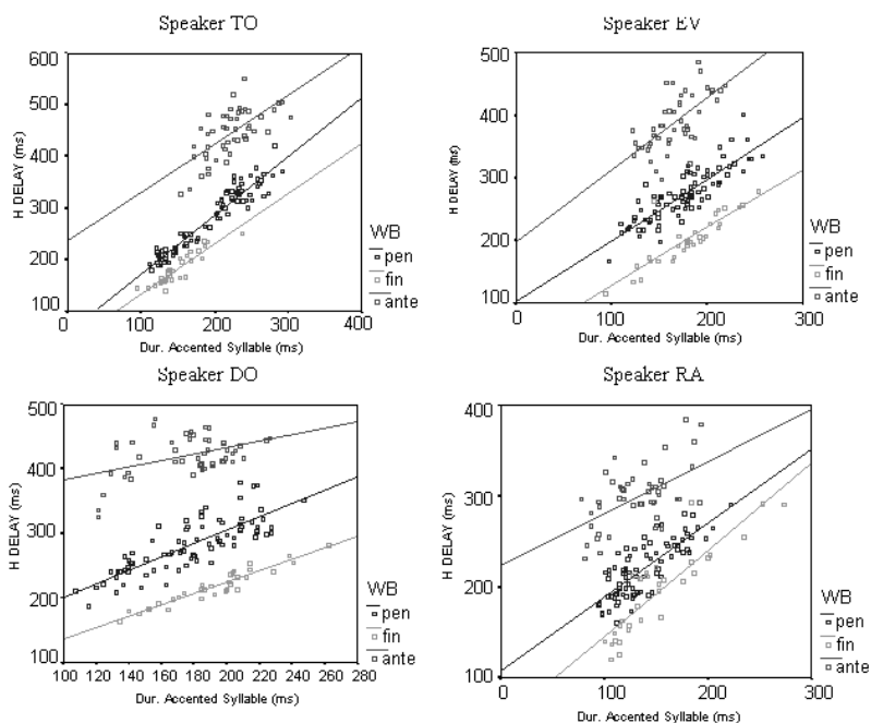
Figure 3. Peak delay (or distance between the onset of the accented syllable and the F0 peak) in ms as a function of the duration of the accented syllable in ms in three stress conditions (words with final, penultimate and antepenultimate stress) for speakers TO, EV, DO and RA.
